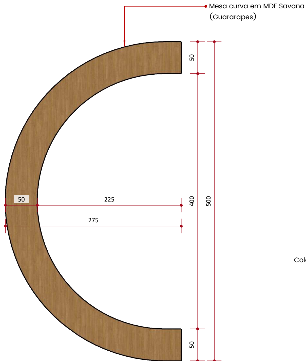
VISTA SUPERIOR MESA
