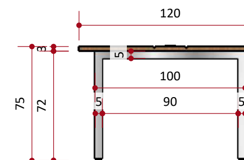
VISTA FRONTAL MESA
