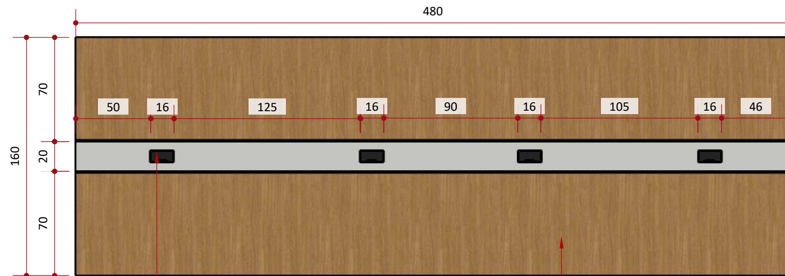
VISTA SUPERIOR MESA
