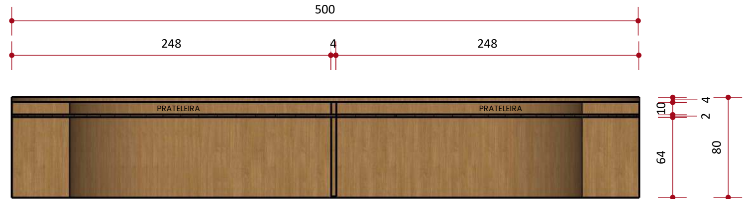
VISTA FRONTAL MESA
