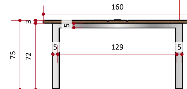
VISTA FRONTAL MESA
